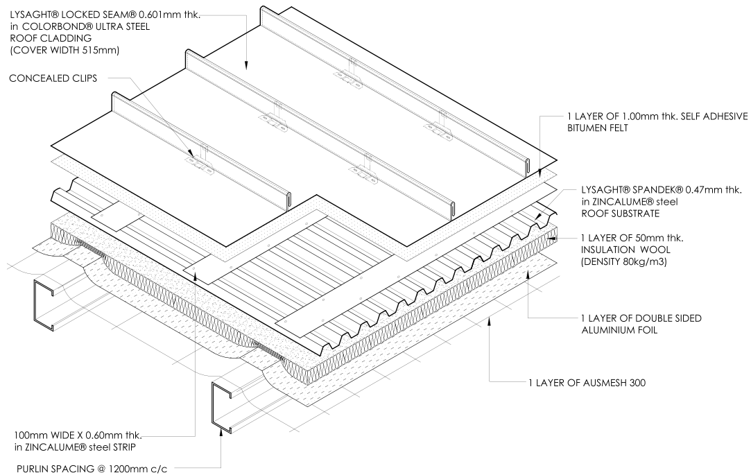
Figure 2: Double Skin Insulated Roof Systems Typical Built-up
