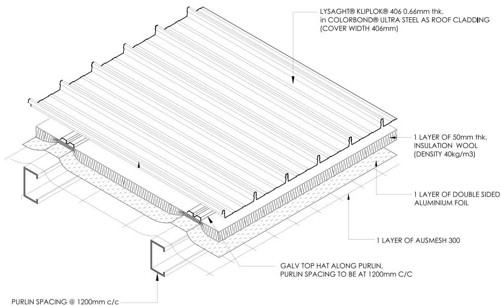
Figure 1: Single Skin Insulated Roof Systems Typical Built-up
