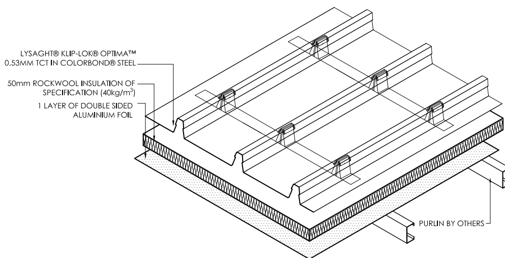
Figure 1: Single Skin Insulated Roof Systems Typical Built-up
