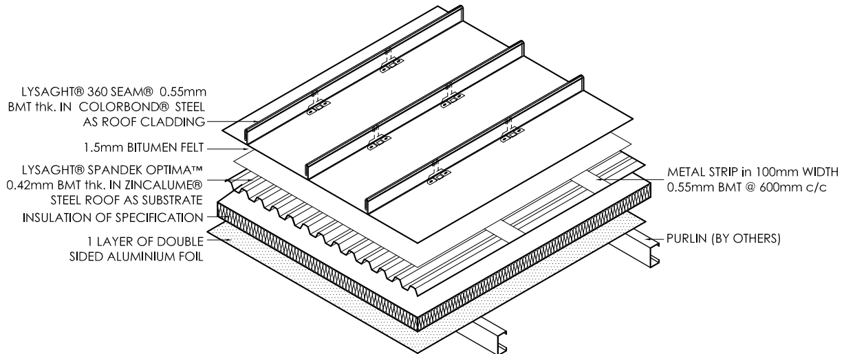
Figure 2: Double Skin Insulated Roof Systems Typical Built-up
